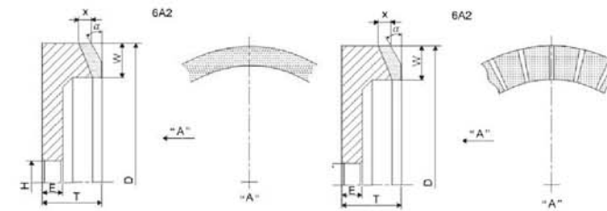
杯型金刚轮 Diamond cup wheel
