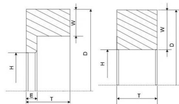
抛光轮 Polishing wheel
