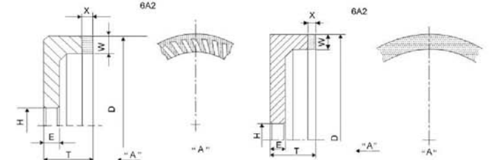
杯型树脂轮 Resin cup wheel
